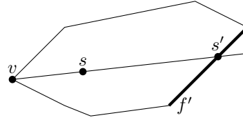
Figure 1 Illustration of one iteration of the GLS method. The point s is a convex combination of the vertex v and the new point s' , which lies on a lower-dimensional face of the polytope, f' .
