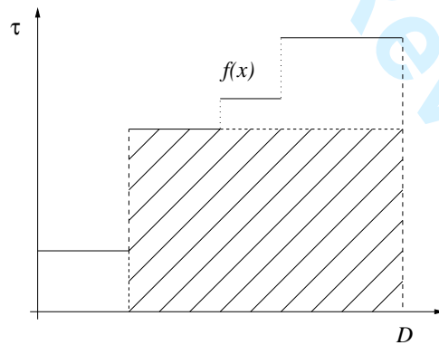
Figure 5. Staircase function f(x) with inscribed maximal rectangle.
