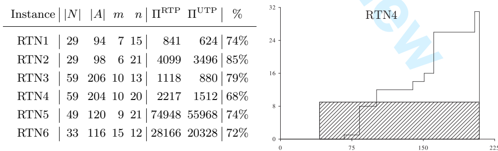
Figure 2.3: Uniform pricing on France Télécom instances.
