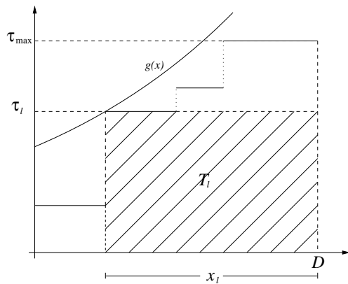
Figure 6. Illustration for the proof of Theorem 4.
